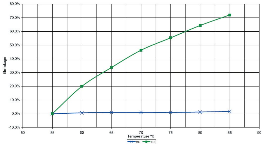
EarthFirst® PLA - TDO film 50µ Shrinkage 10 seconds exposure in water
